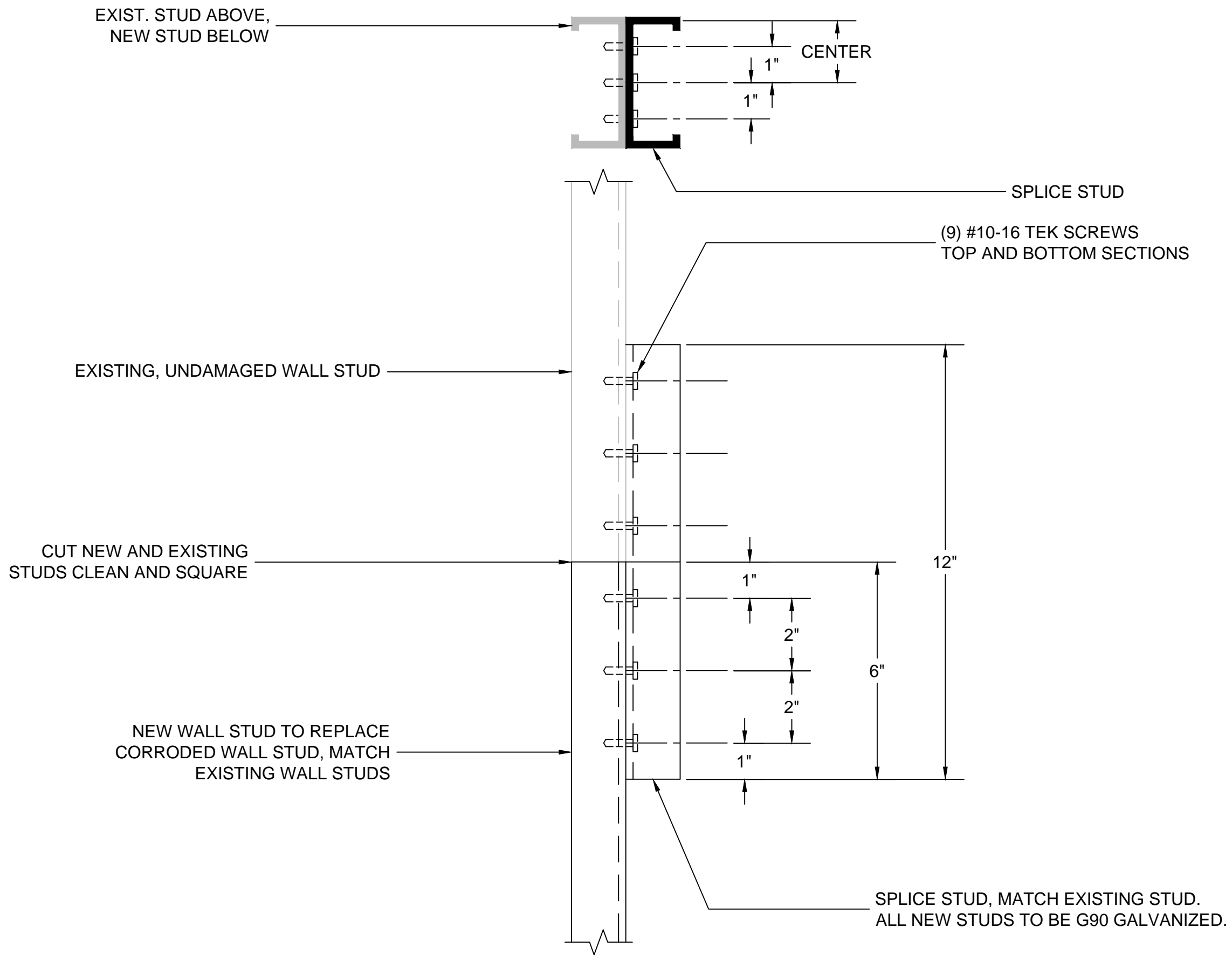
TYPICAL LIGHT GAUGE METAL STUD SPLICE DETAIL
